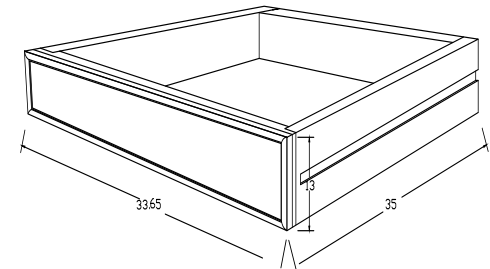
DETAIL DRAWER
